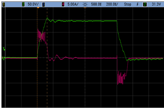
Figure 21. Current and Voltage Traces from Piezo IPhaseArray Configuration Example 2
