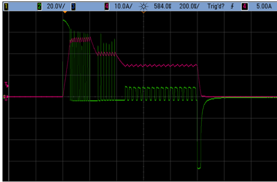
Figure 6. Solenoid IPhaseArray Configuration Example 3
