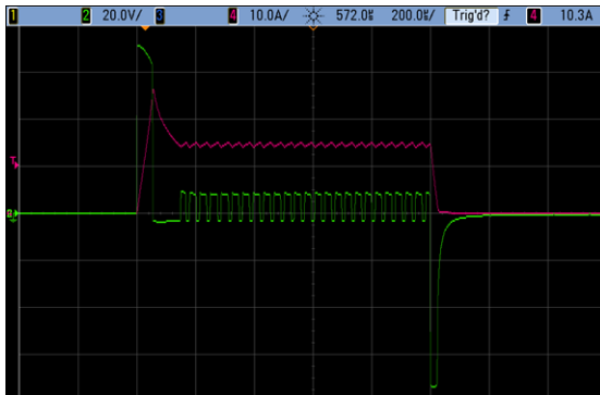
Figure 10. Current and Voltage Traces from Phase1FirstPeakEnable=TRUE Operating Mode
