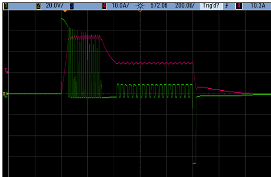
Figure 12. BackBoostTime = 0.025 ms
