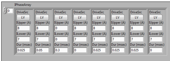
Figure 26. Piezo IPhaseArray Configuration Example 5
