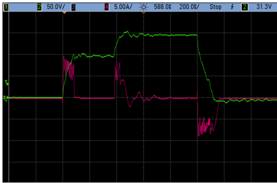
Figure 27. Current and Voltage Traces from Piezo IPhaseArray Configuration Example 5
