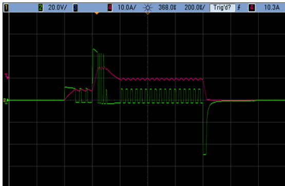
Figure 7. Current and Voltage Traces from Solenoid IPhaseArray Configuration Example 3
