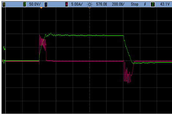
Figure 25. Current and Voltage Traces from Piezo IPhaseArray Configuration Example 4
