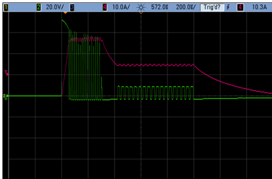
Figure 12. BackBoostTime = 0.025 ms
