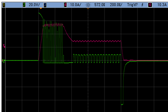
Figure 15. BackBoostTime = 0.150 ms
